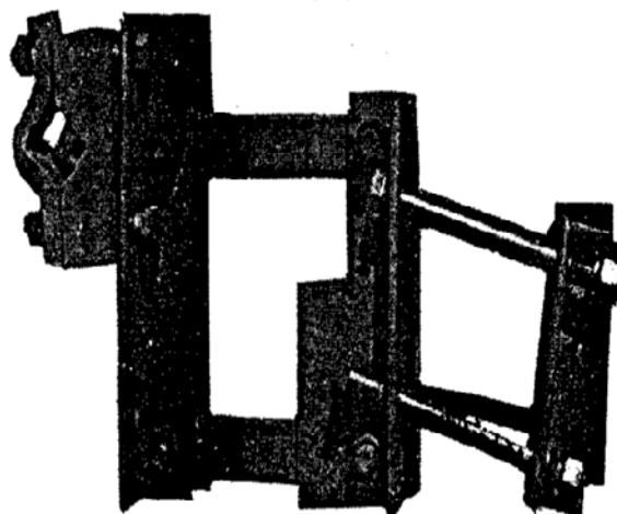
Bumble Bee Hitch 4½ x 7½ inch bar to 2¼ inch bar.
