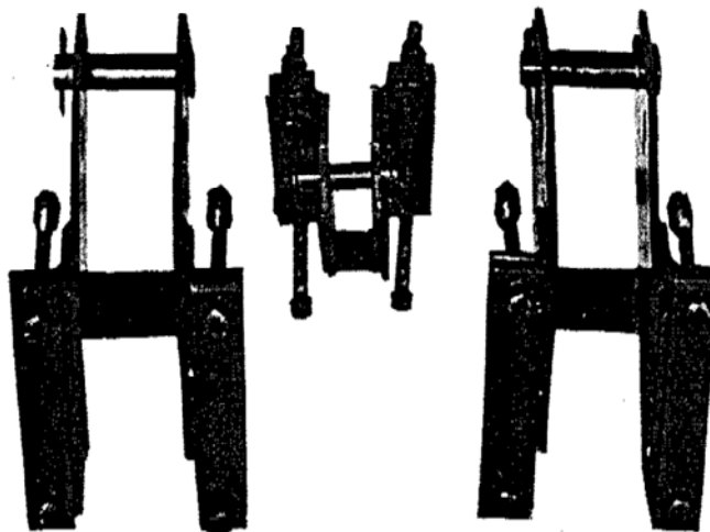
Bumble Bee Hitch 4½ x 7½ inch bar to 2¼ inch bar.
